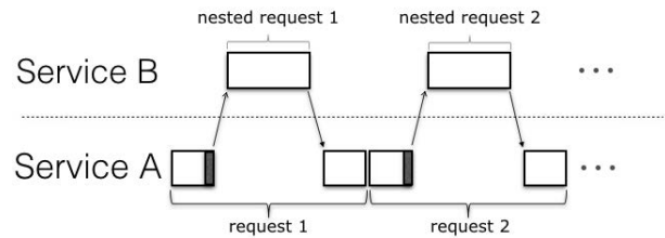
Figure 2. Sequential execution of requests in a multi-service setting. Bound by sequential execution, service A must remain idle while its nested requests are being processed at service B .
