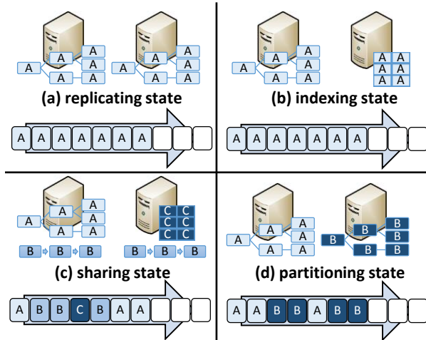
Figure 5: Use cases for Tango objects: application state can be distributed in different ways across objects.
